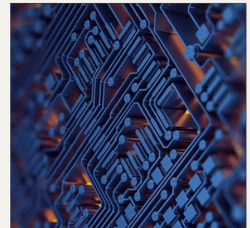
Monotone Fuzzy Systems
